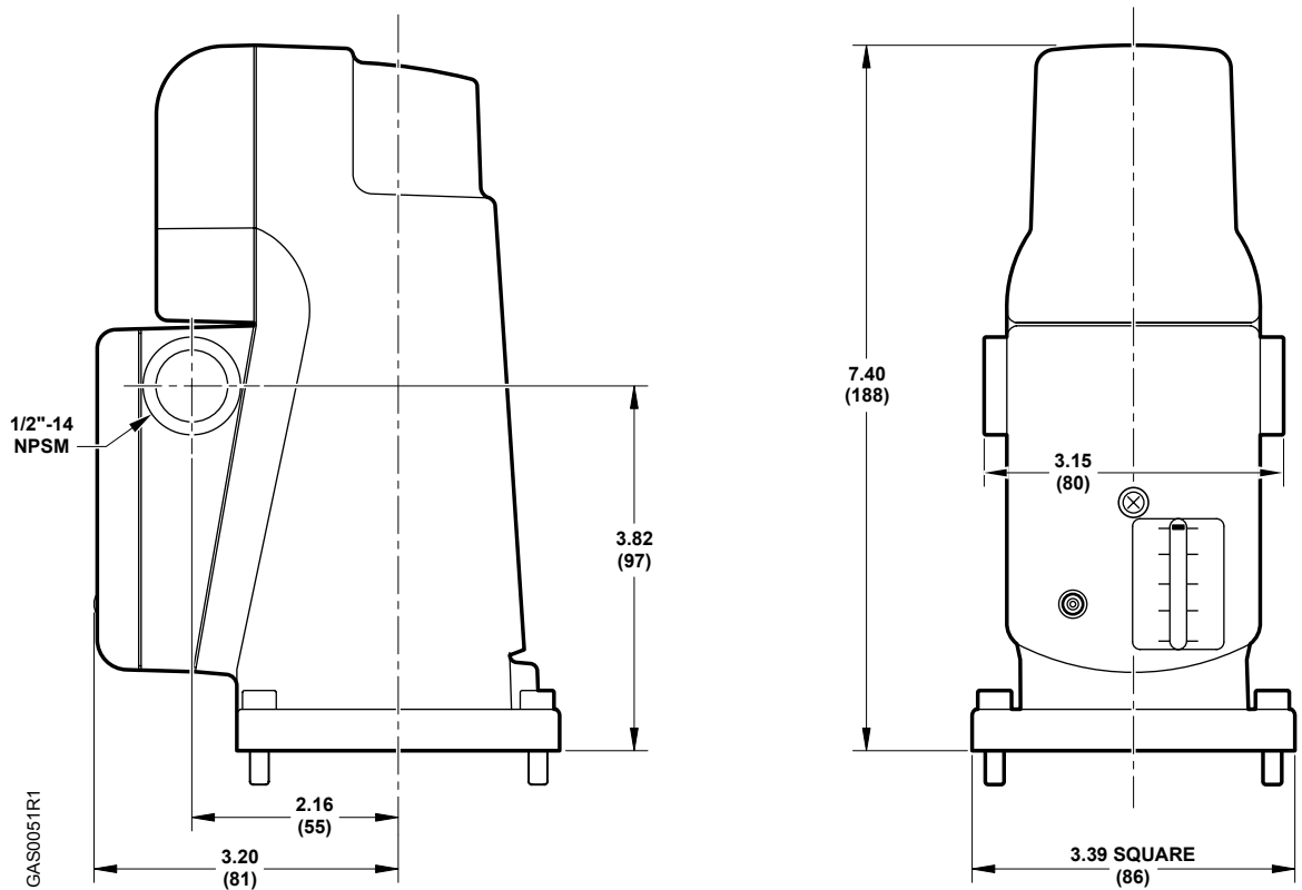
Figure 3. SKP15...U.. Dimensions.
