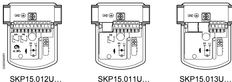
Figure 2. Terminal Designations.
