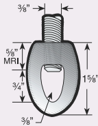
Coupler Nut
