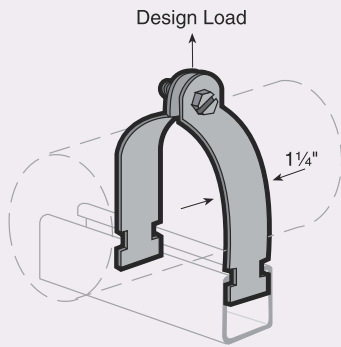
Pipe Clamp
