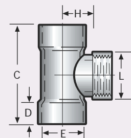
Adapter Tee
