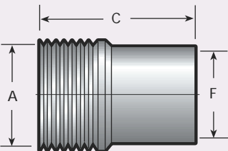
Male Adapter
