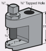
Beam Clamp
