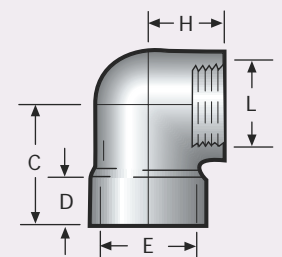
90° Adapter Elbow
